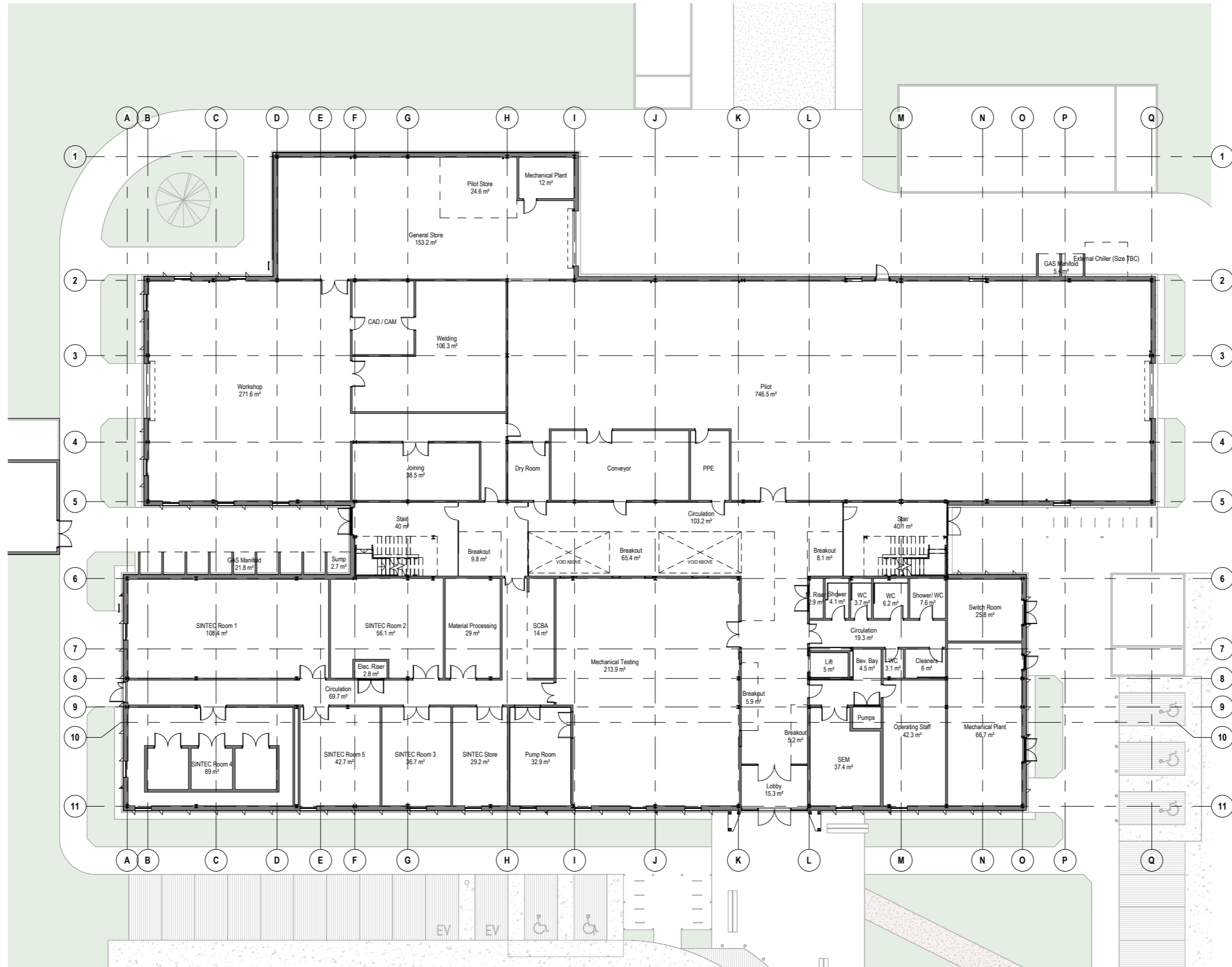
GA Plan - Level 00
