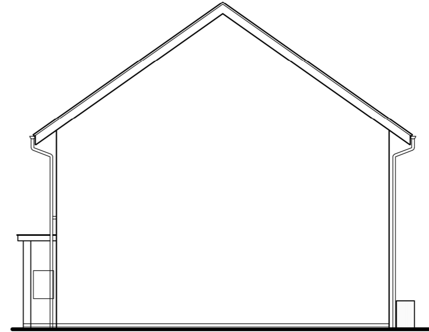
GABLE ELEVATION
