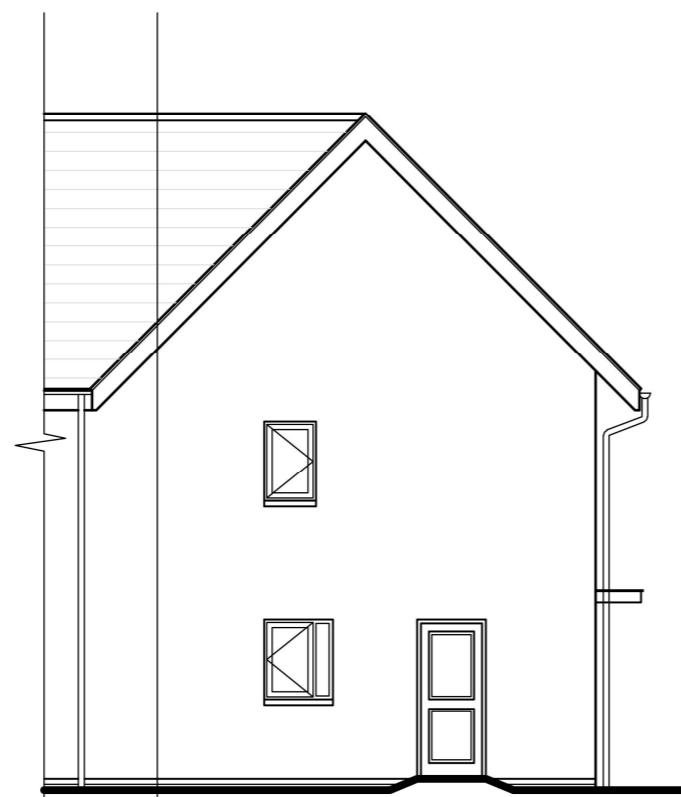
Rear Elevation
