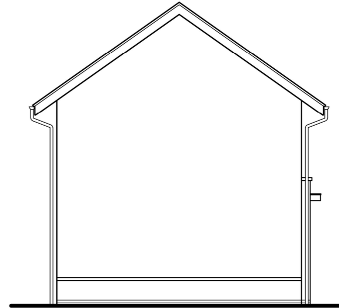
Gable Elevation
