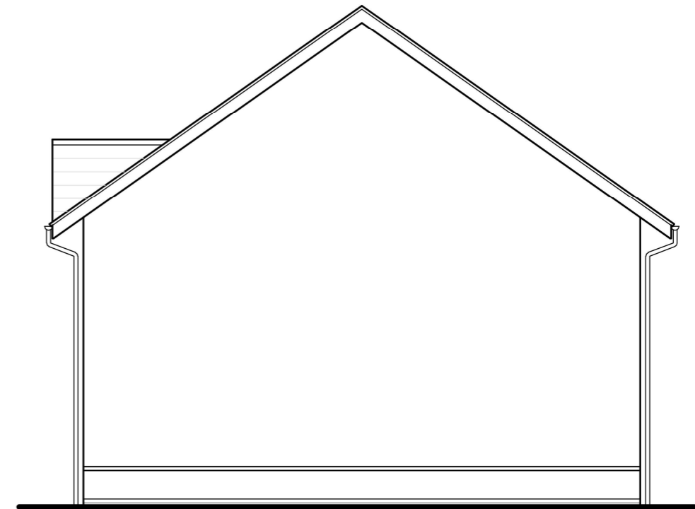
Gable Elevation
