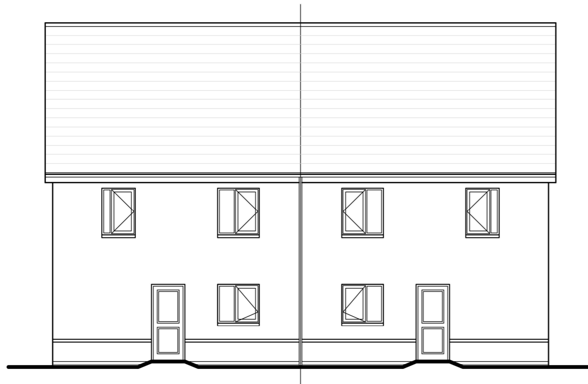
Rear Elevation
