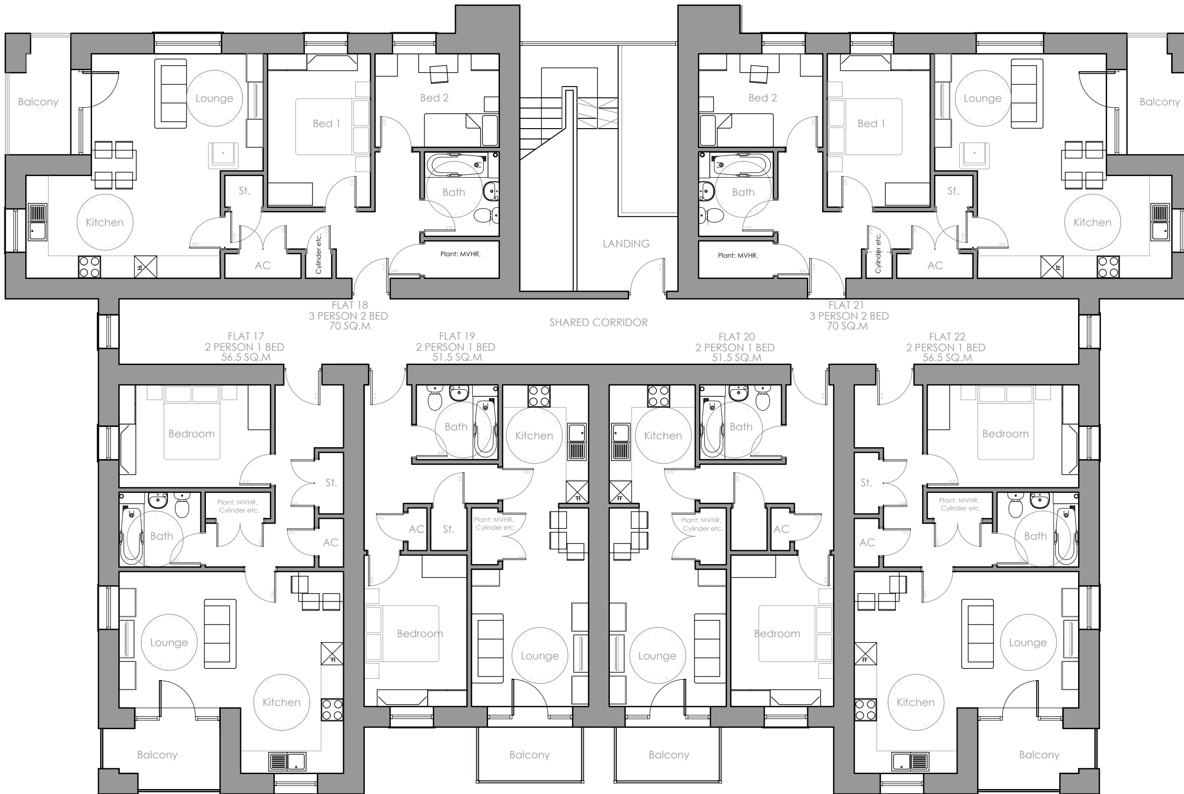
SECOND FLOOR
