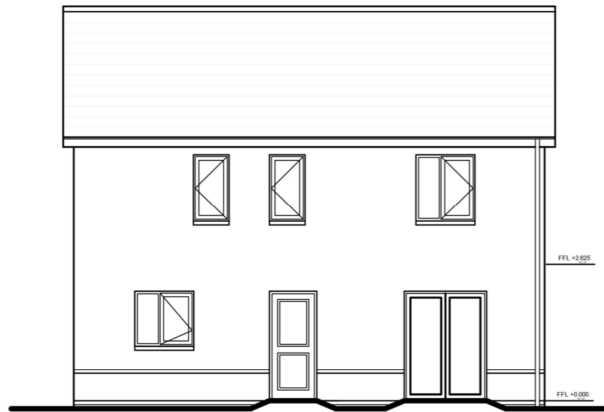
Rear Elevation
