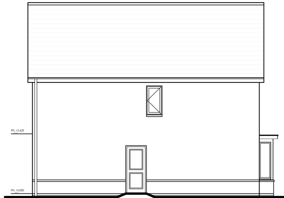
Rear Elevation
