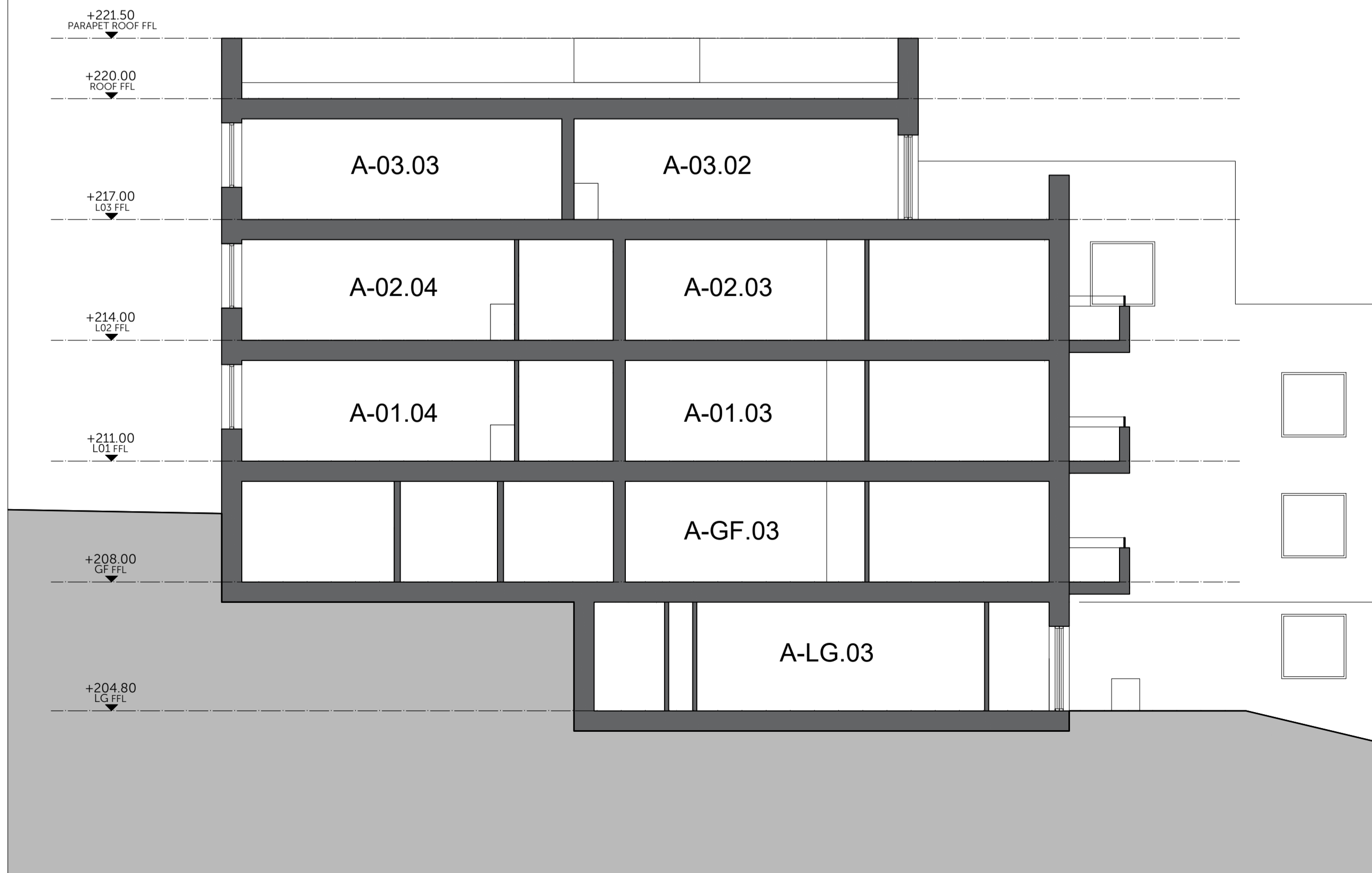
2 BLOCK A SECTION BB
