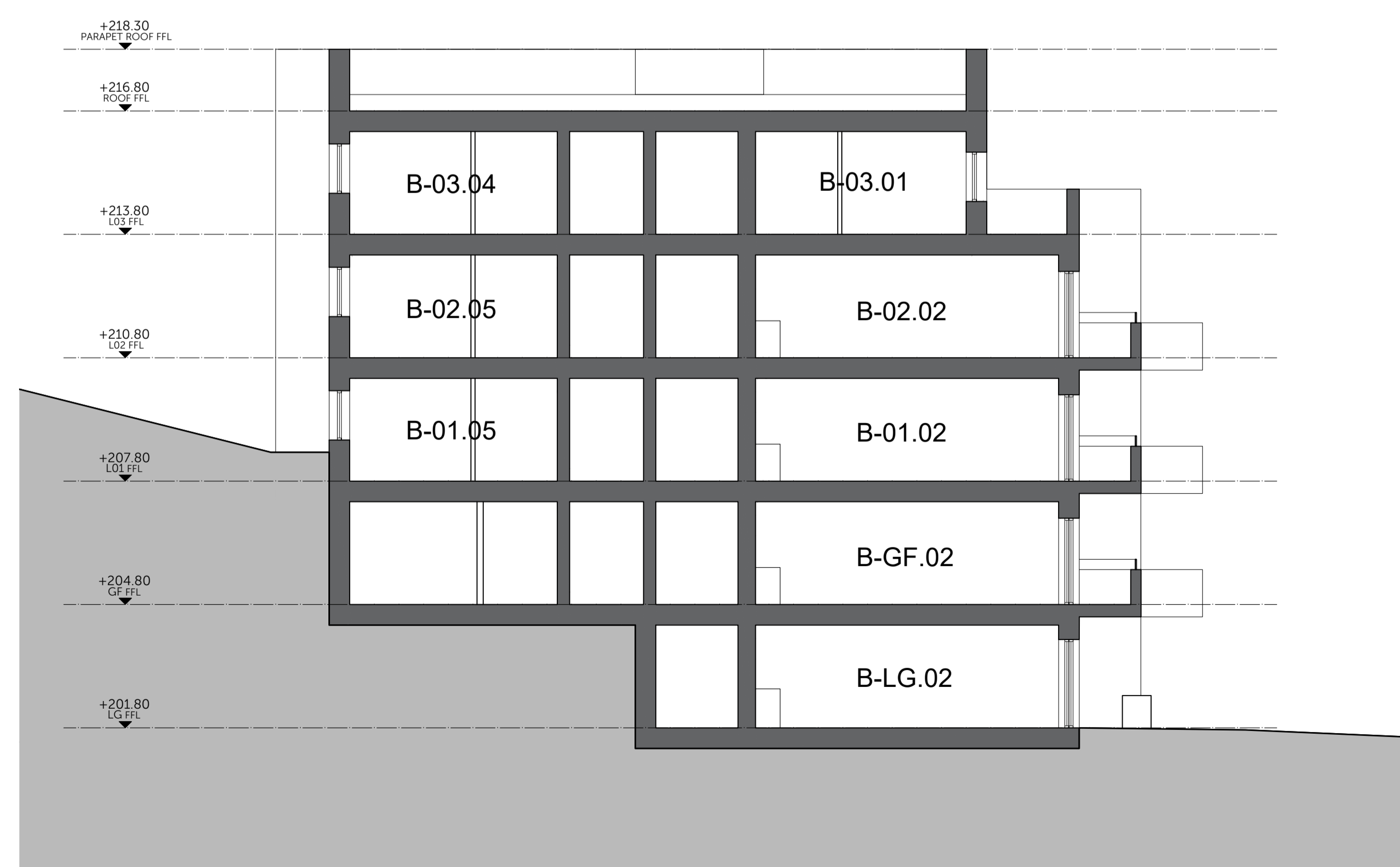
3 BLOCK B SECTION CC
