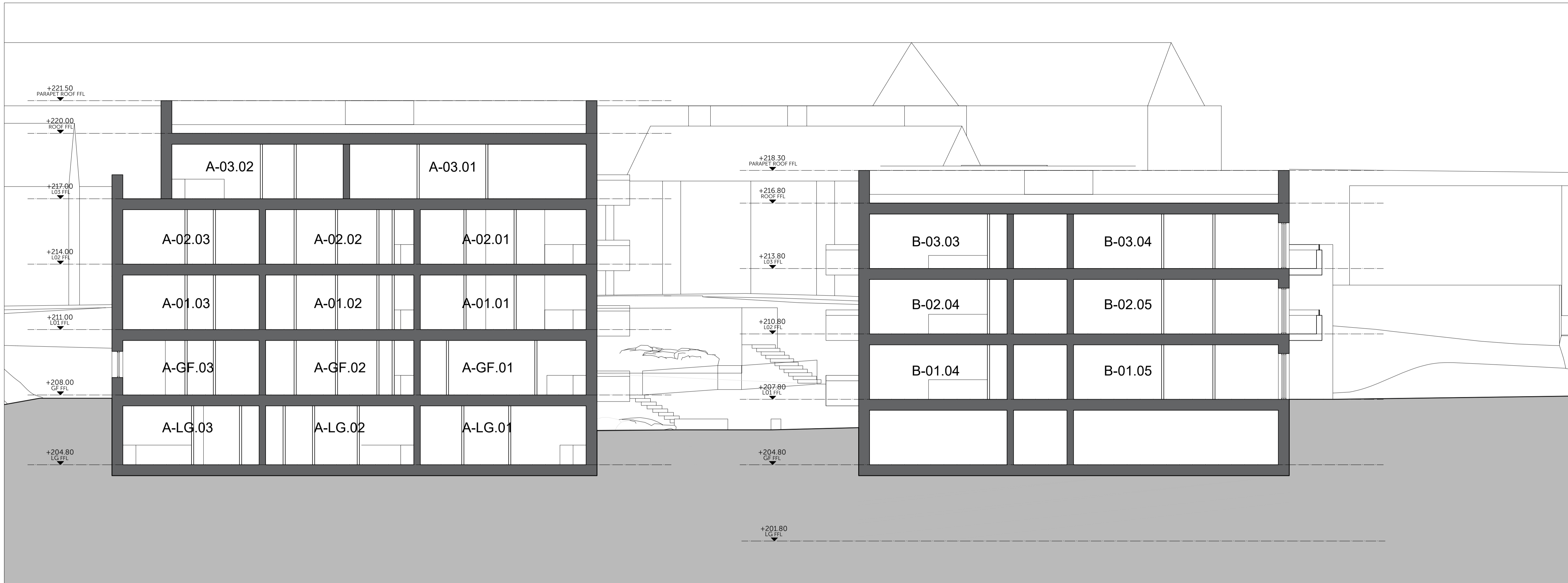
1 LONG SECTION AA
